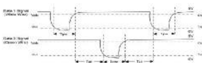
Figure 1 Sequence Diagram
