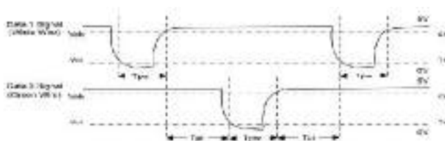
Figure 1 Sequence Diagram
